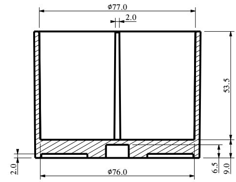
SECTION Y-Y
