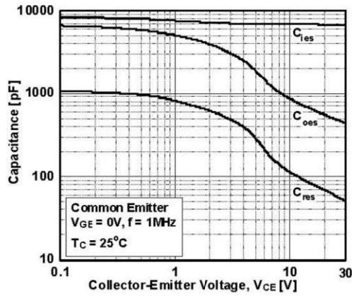
Capacitance Characteristics
