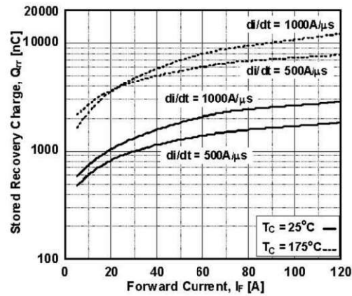
Stored Charge
