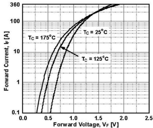
Forward Characteristics
