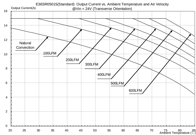
Figure 22: Output current vs. ambient temperature and air velocity @ V_{in}=24V (Transverse Orientation)
